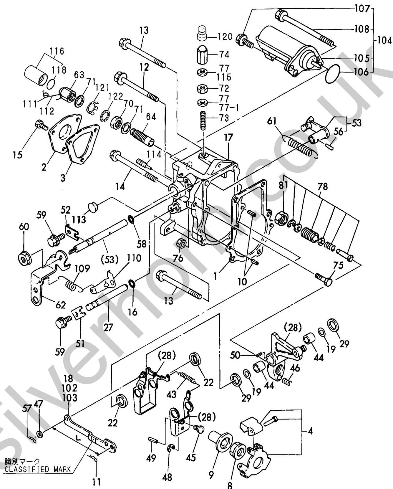
Fig. 12 ガバナ GOVERNOR
